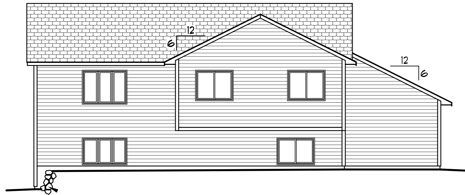
REAR ELEVATION
