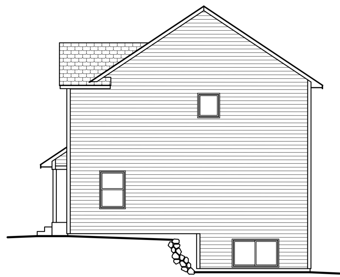
ELEVATION "A"
